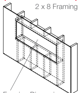
Framing Dimensions
